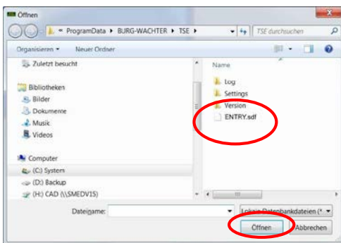
Abb. 44: Explorer
