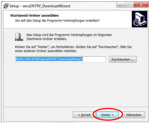
Abb. 8: Setup DownloadWizard
