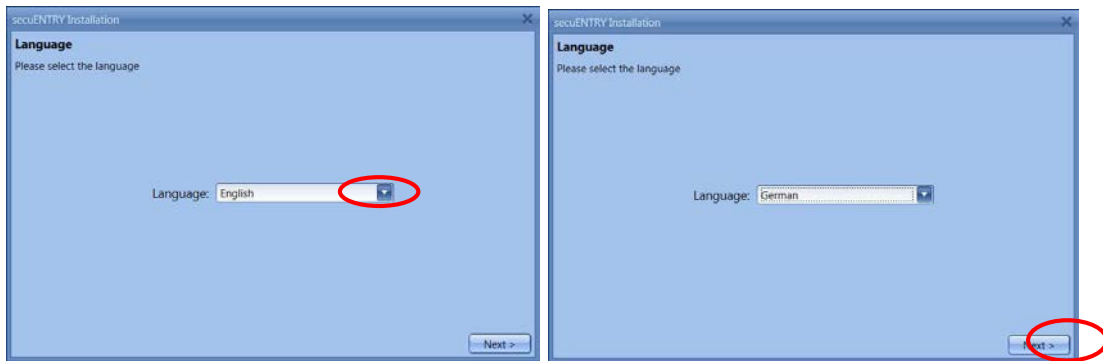
Abb. 23: Setup Software
